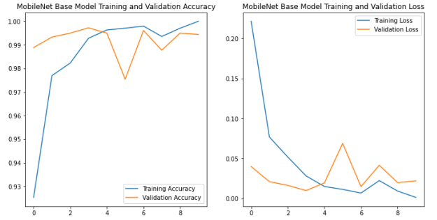
Fig. 6. The MobileNet Base Model: (a) Accuracy (b) Loss Graph.
