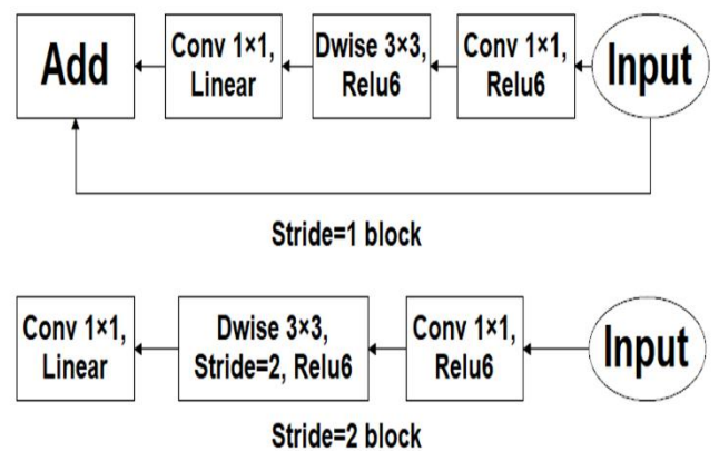
Fig. 5. Proposed Method MobileNetV2 Architecture.
