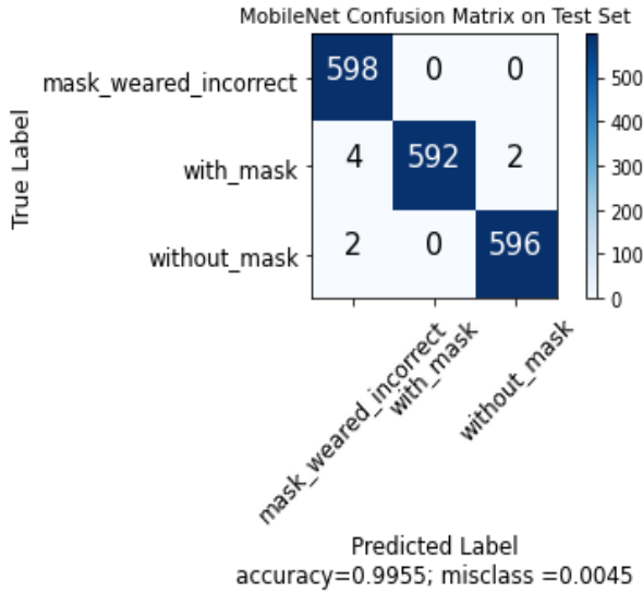
Fig. 7. The MobileNet Base Model Confusion Matrix on Test Set.
