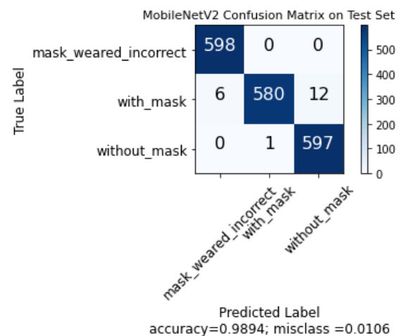
Fig. 9. The MobileNetV2 Base Model Confusion Matrix on Test Set.
