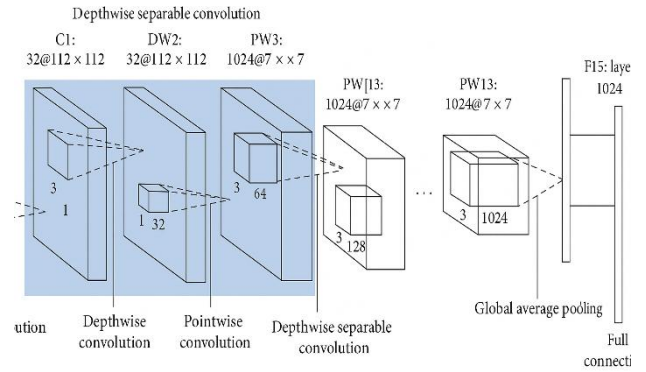
Fig. 4. Proposed Method MobileNet Architecture.
